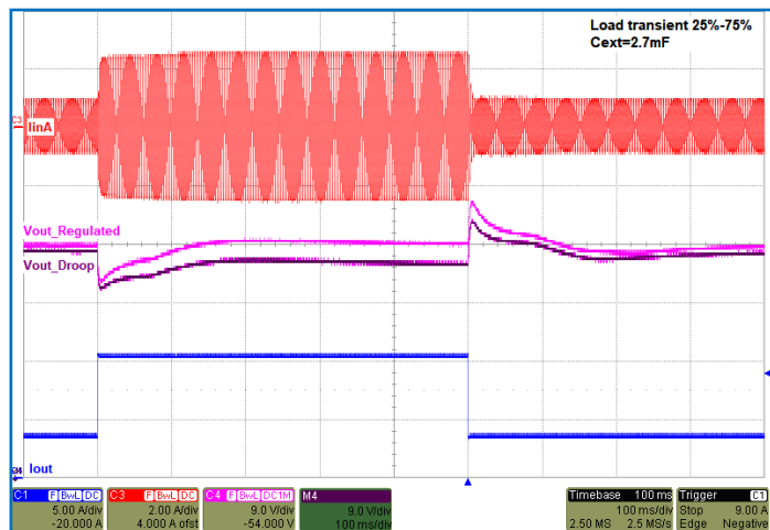
Figure 10: Responses to 25%-75%-25% Load Transient Steps: Cext=10mF, both Regulated and Droop models.
